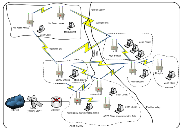
Figure 4: Mesh network at Pebbles valley
